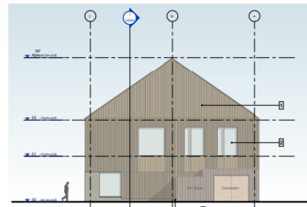
3 Proposed East Elevation 1:100
