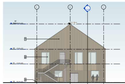
5 Proposed West Elevation 1:100
